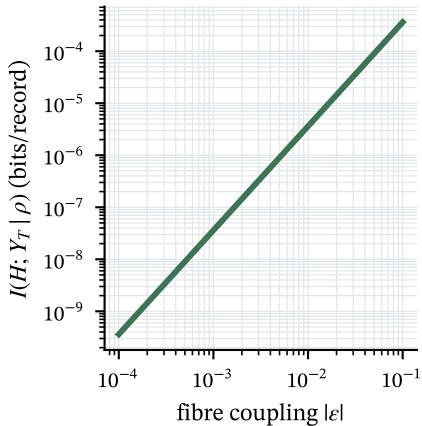
History-information witness
